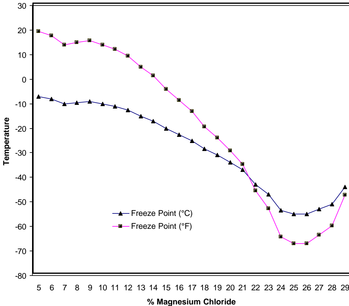
Ice Ban 300 Phase Diagram
